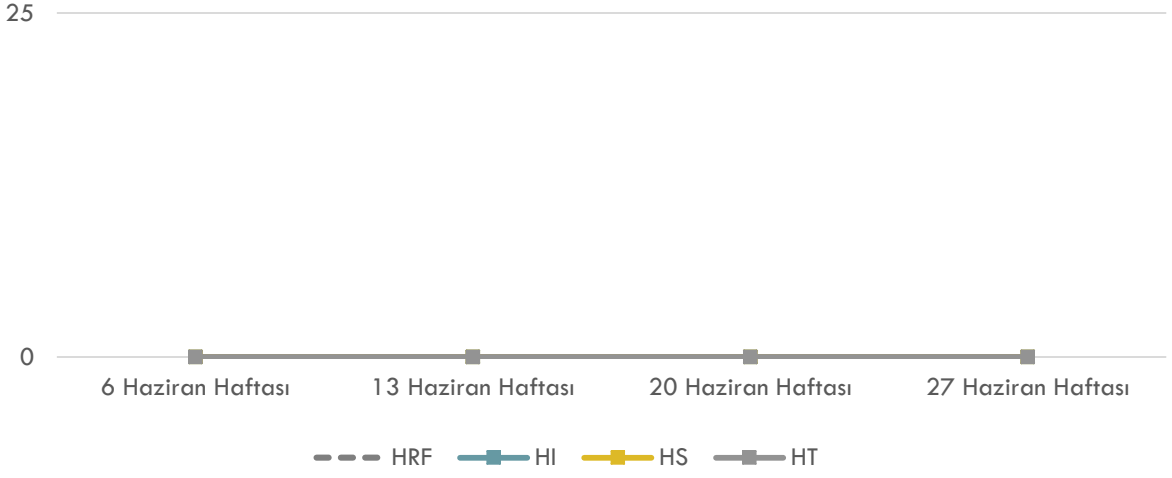
Haziran 2022 HRF - HI - HS - HT (TL/'000 Sm 3 )
