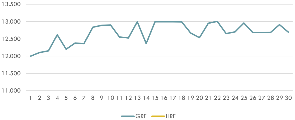
Haziran 2022 GRF - HRF (TL/'000 Sm 3 )
